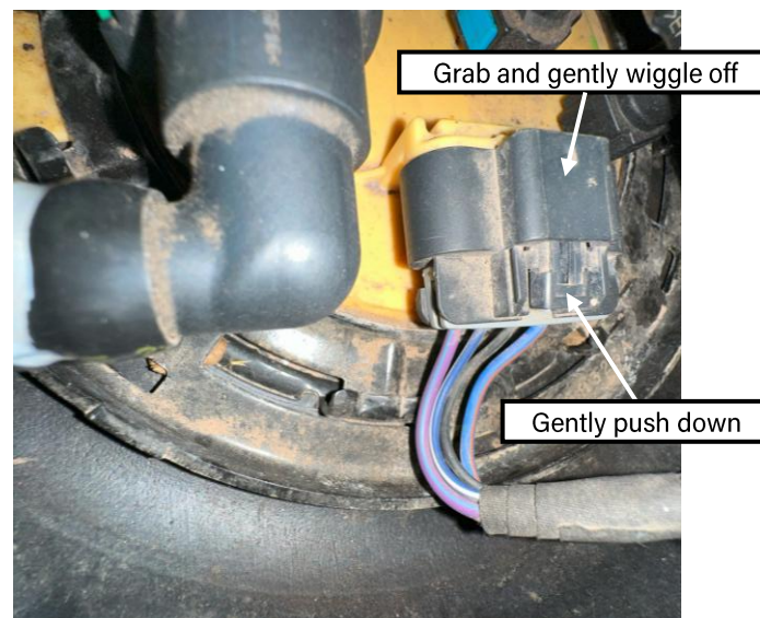
Figure 7: wiring harness
