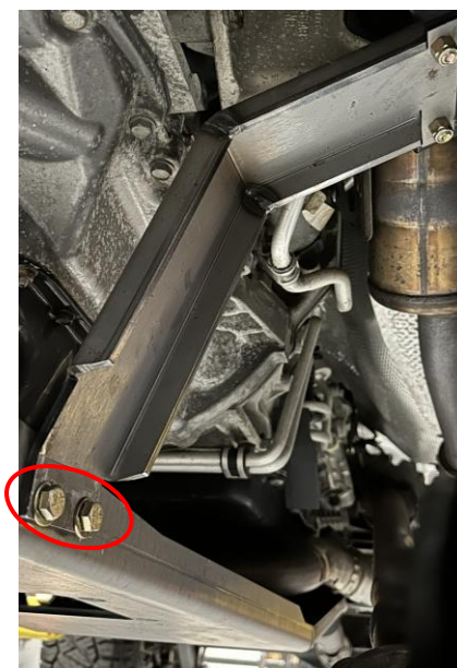
Figure 37: New skid plate installed at OEM 3.6L motor mount locations and skid plate connections
