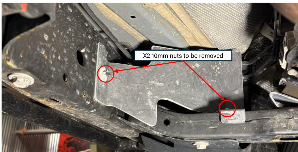
Figure 3: Plastic fuel line guard to be removed temporarily
