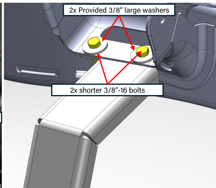
Figure 34: CAD and installation of driver-side motor mount bracket
