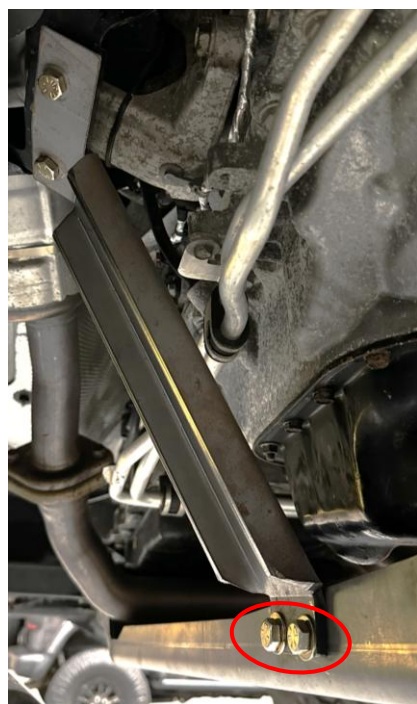
Figure 37: New skid plate installed at OEM 3.6L motor mount locations and skid plate connections
