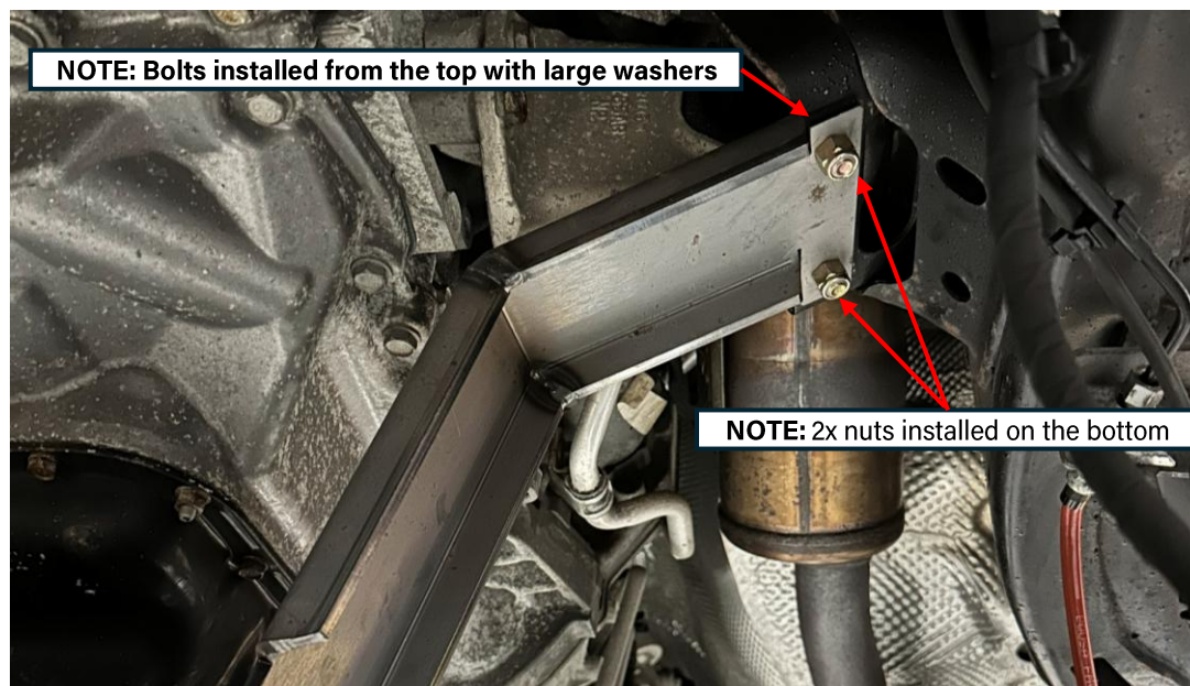
Figure 34: CAD and installation of driver-side motor mount bracket
