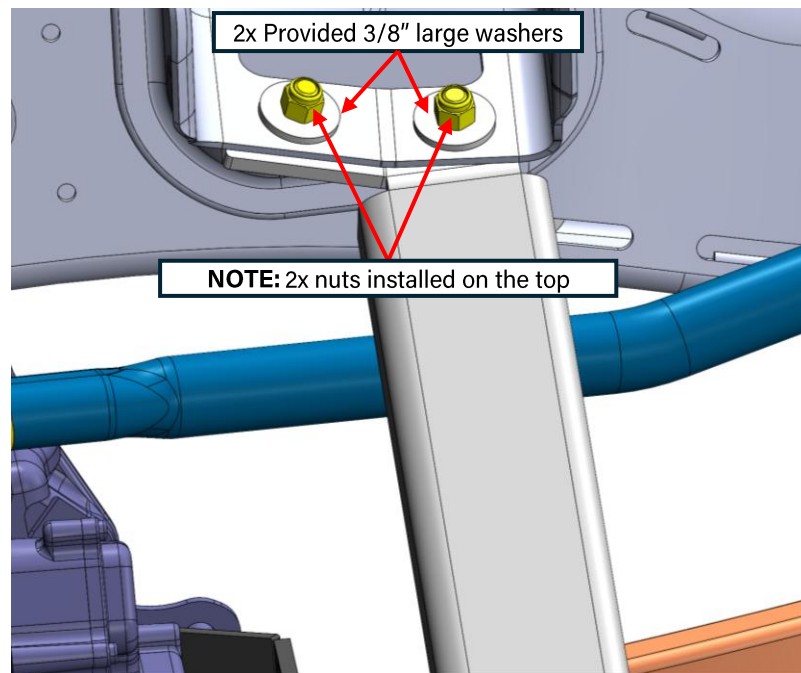
Figure 35: CAD and installation of passenger side motor mount bracket
