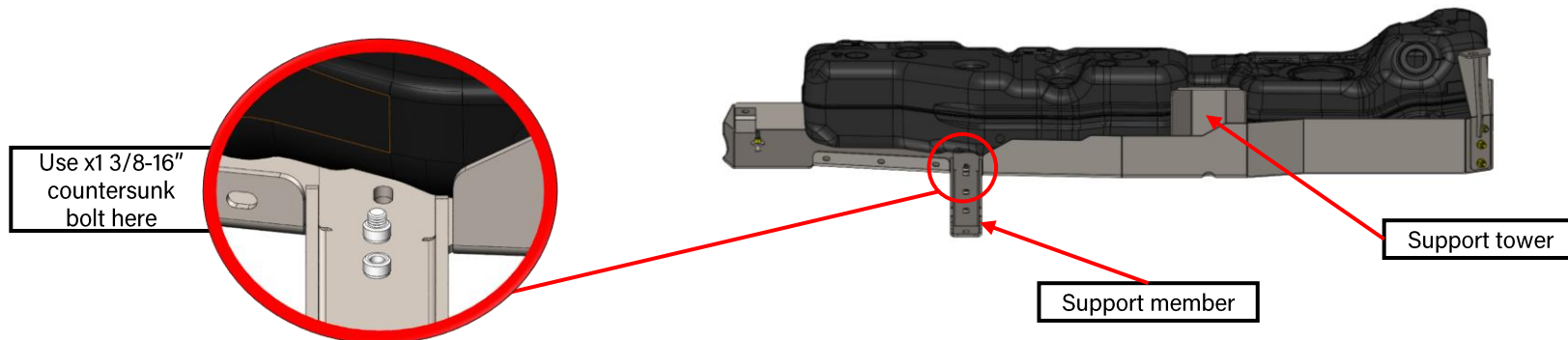
Figure 15: Gas tank installed into the skid plate with the support member underneath
