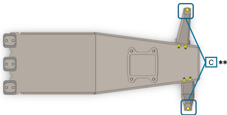
Figure 44: bolt callouts on engine skid plate
