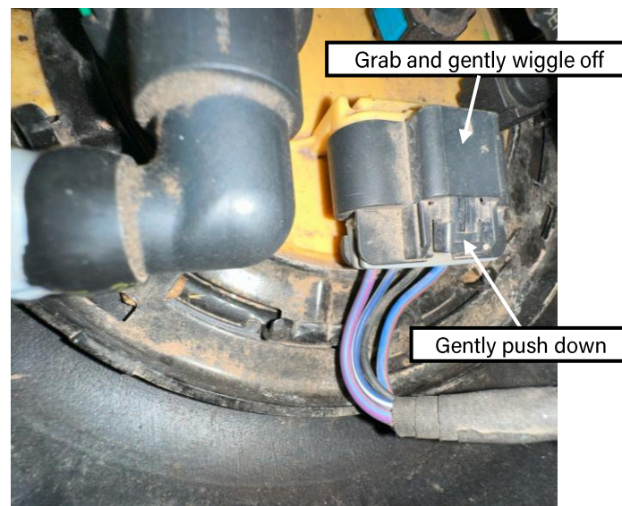
Figure 7: wiring harness
