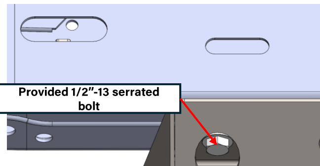
Figure 30: Drilling 17/32" frame rail hole for the provided 1/2"-13 serrated bolt and flagnut
