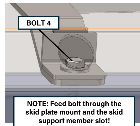
Figure 20: Bolt 4
