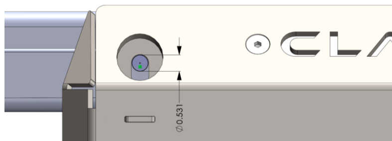
Figure 30: Drilling 17/32" frame rail hole for the provided 1/2"-13 serrated bolt and flagnut
