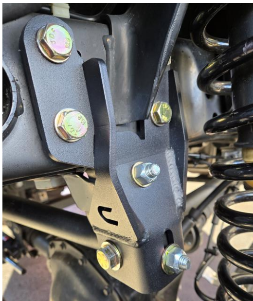
Figure 7: Bracket installed
