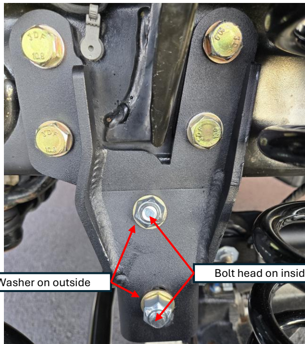
Figure 6: Centering bolts installed (top bolt is left loose)
